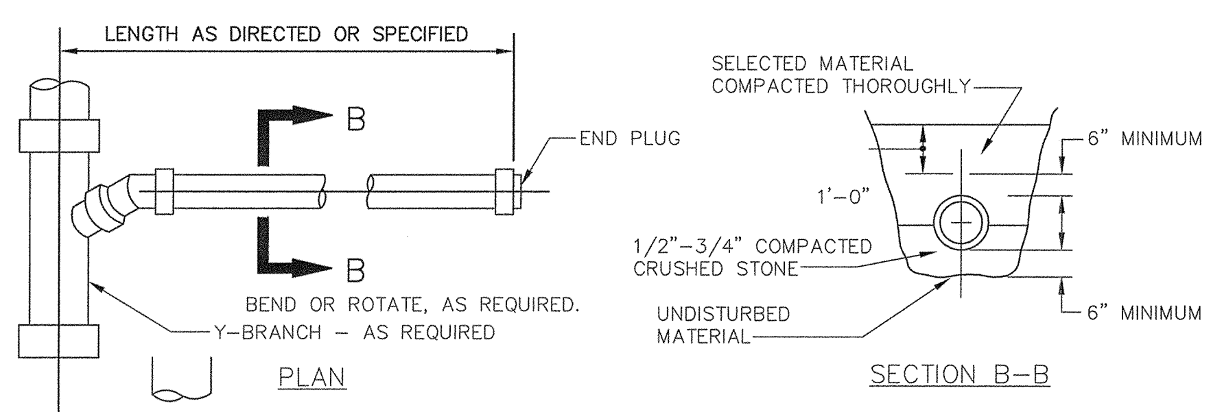
TYPICAL BUILDING CONNECTION NOT TO SCALE
