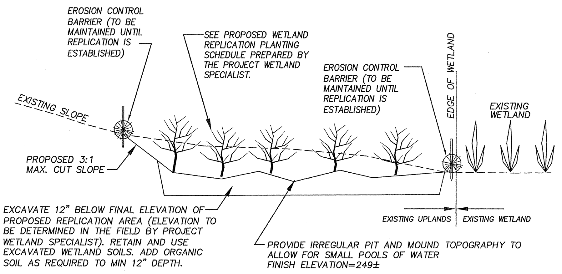
WETLAND REPLICATION AREA CROSS-SECTION NOT TO SCALE
