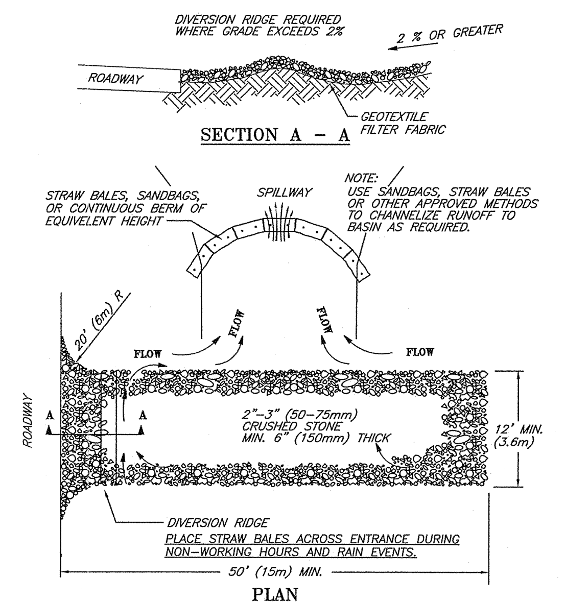
TEMPORARY GRAVEL CONSTRUCTION ENTRANCE/EXIT © 1994 JOHN MCCULLAN
