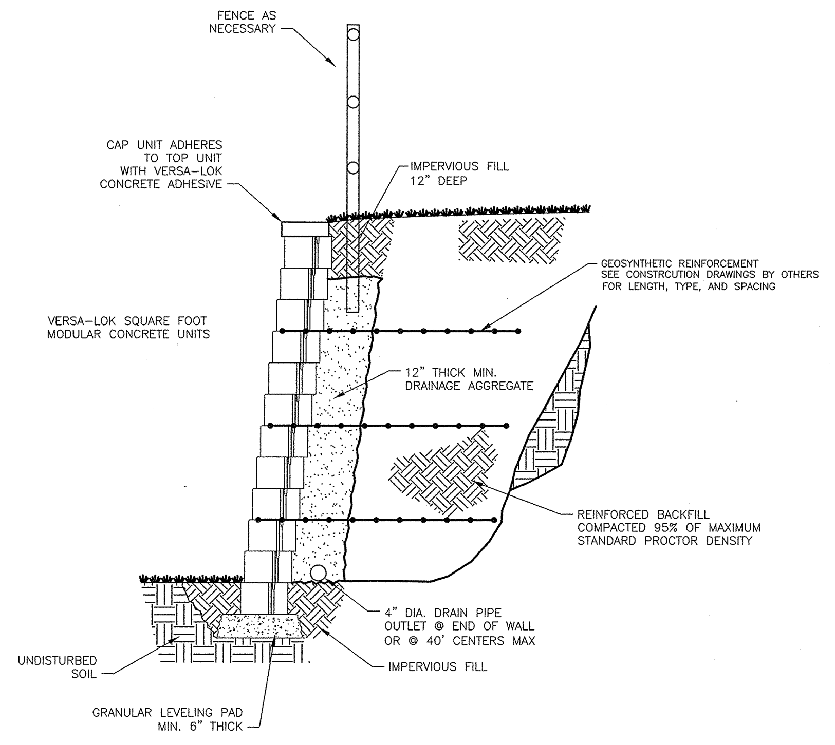
TYPICAL SECTION REINFORCED RETAINING WALL SCALE: NONE
