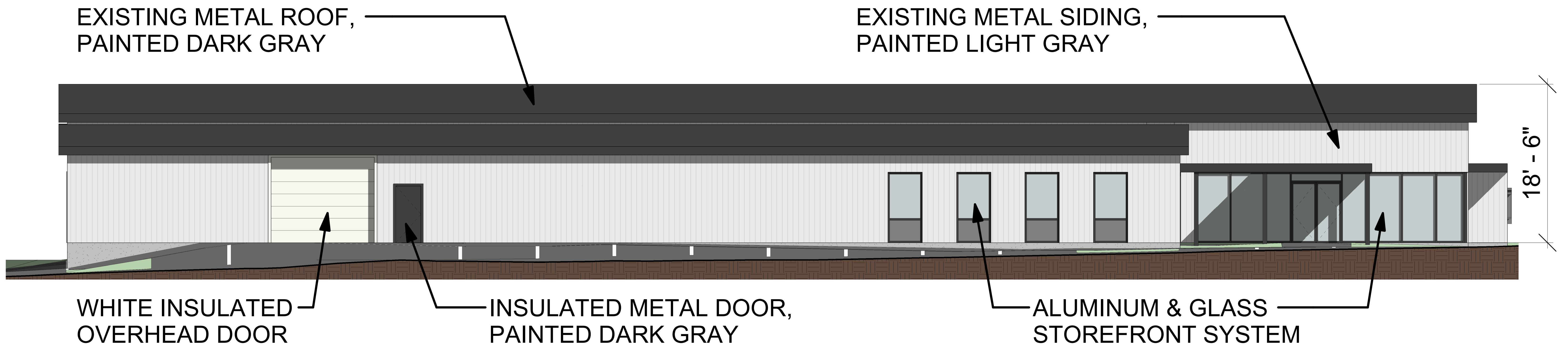
EAST ELEVATION
